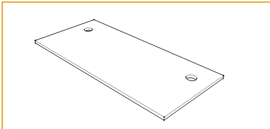
1500mm W x 700mm D x 25mm
